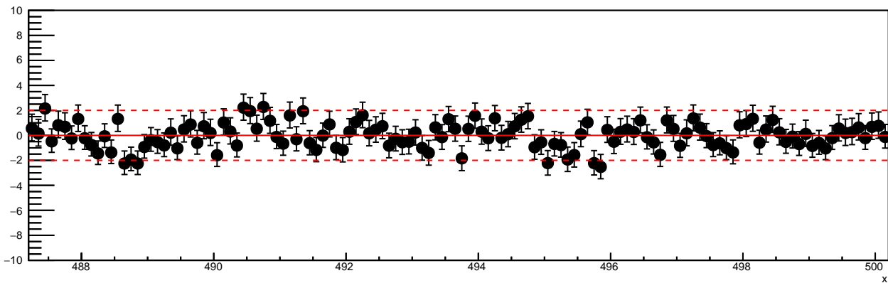
Pulls bin-by-bin
