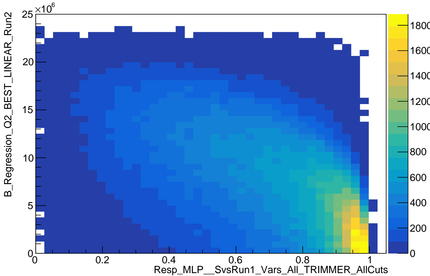
B_Regression_Q2_BEST_LINEAR_Run2:Resp_MLP__SvsRun1_Vars_All_TRIMMER_AllCuts
