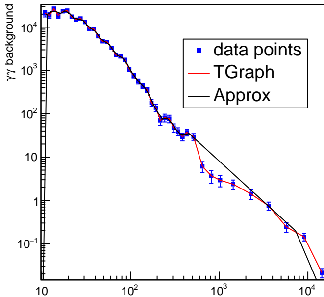
Approx: "linear",nout,xout,0,0,0,0,"ordered"
