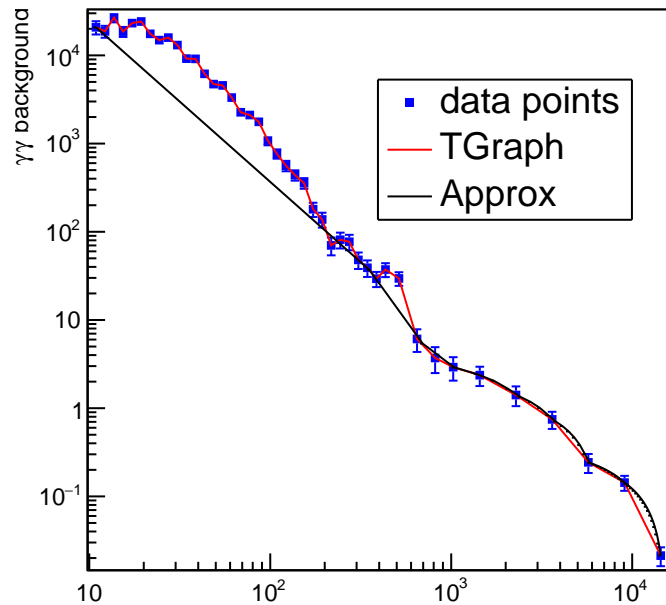
Approx: "linear",0,0,0,0,0,0,"ordered"
