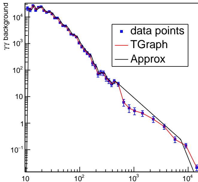
Approx: "constant",nout,xout,0,0,0,0,"ordered"
