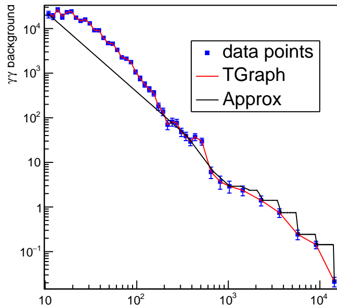
Approx: "constant",0,0,0,0,0,0,"ordered"
