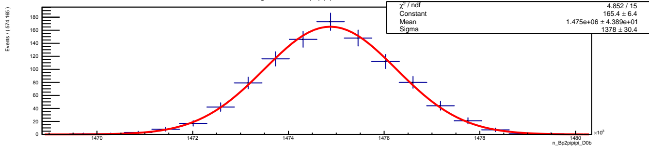
Histogram of __n_Bp2pipipi_D0b
