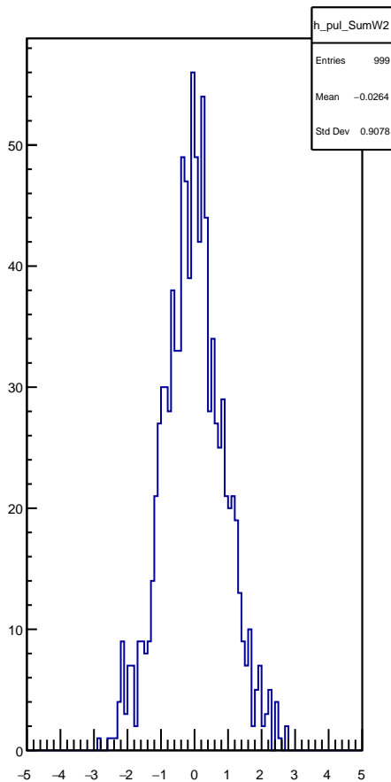
pulls for SumW2
