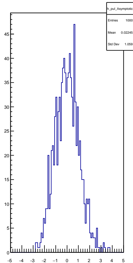
pulls for Asymptotic
