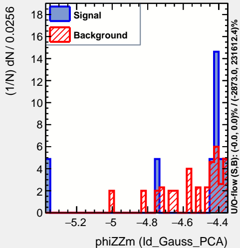
Input variable: phiZZm
