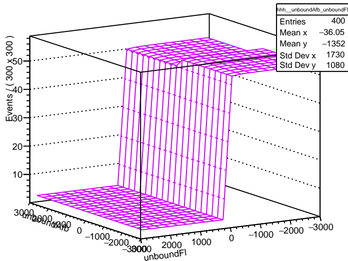
Likelihood Function
