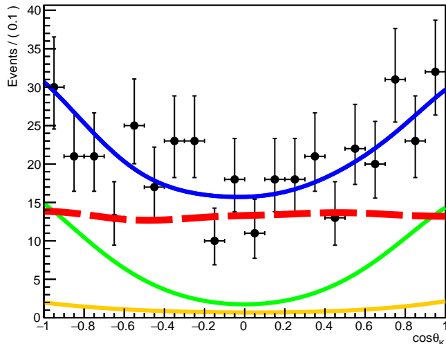
\text{Cos}\theta_K : toy data with best fit model
