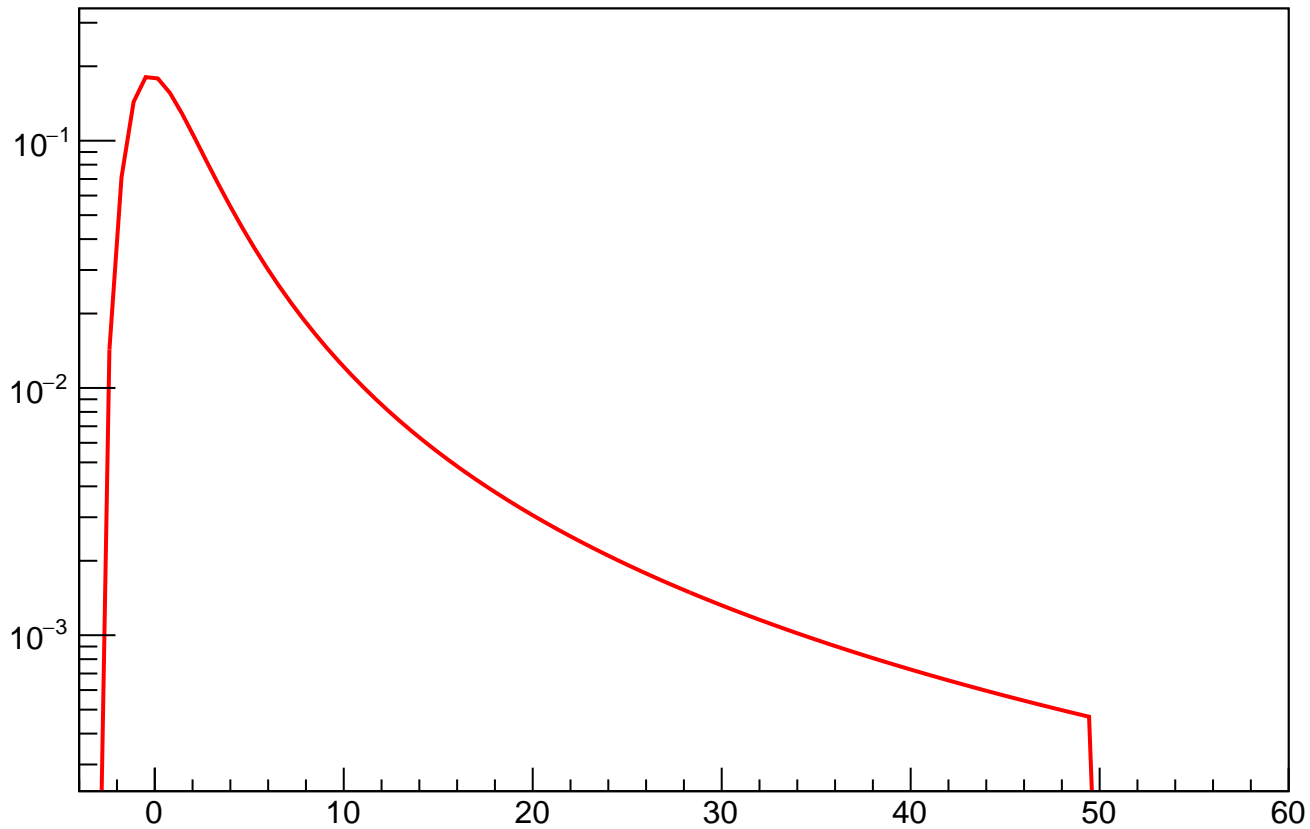
TMath::Vavilov(x, 0.01, 0.5)
