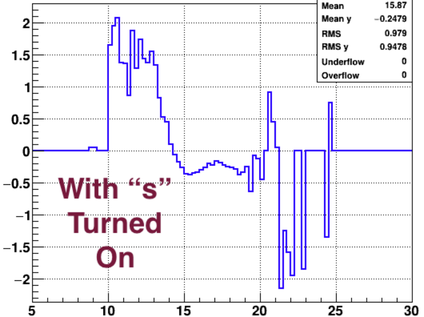
RMS (Spread) ProfileY of tot vs. nSigmaTof( \pi )
