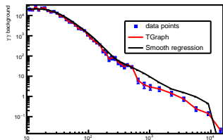
Super smoother: "",0,0,kFALSE,0
