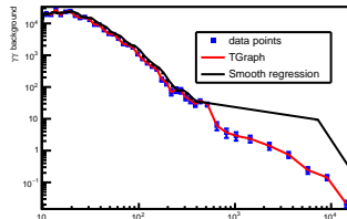
Kernel smoother: "box",2.0,nout,xout
