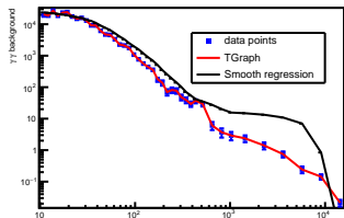
Super smoother: "",0,0.3,kFALSE,0
