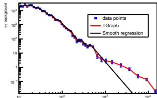
Kernel smoother: "normal",2.0,nout,xout
