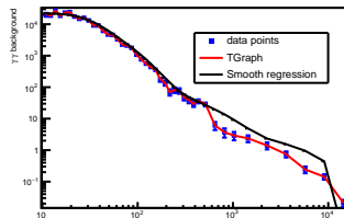
Super smoother: "",3,0,kFALSE,0
