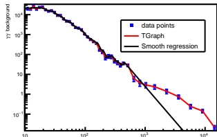
Kernel smoother: "normal",5.0,nout,xout
