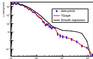
Super smoother: "",3,0.3,kFALSE,0
