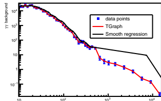
Kernel smoother: "box",5.0,nout,xout
