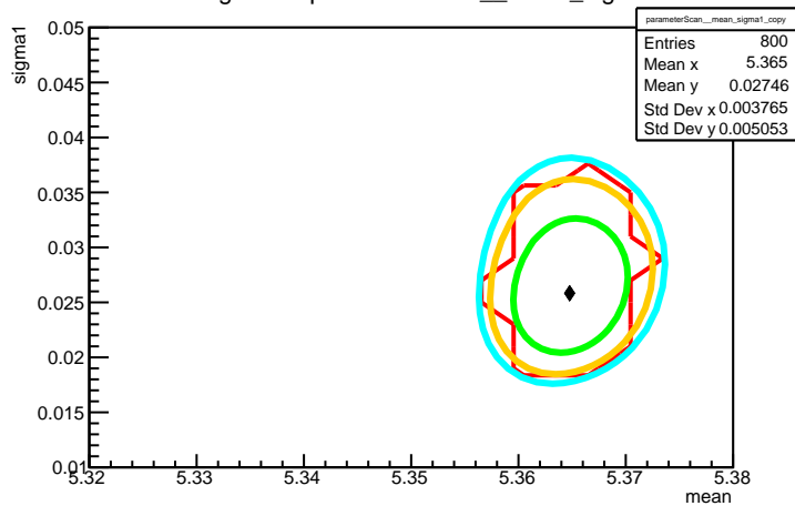
Histogram of parameterScan__mean_sigma1
