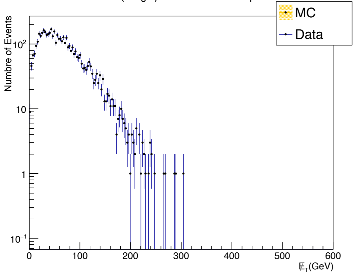
MET Data/MC(Weight) ID== 1 letal< 2.4 mupt > 50 Gev
