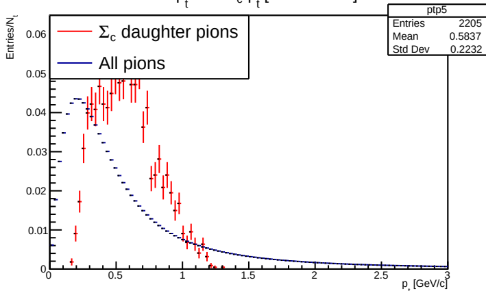
Pion p_t with \Sigma_c p_t [6-12 GeV/c]
