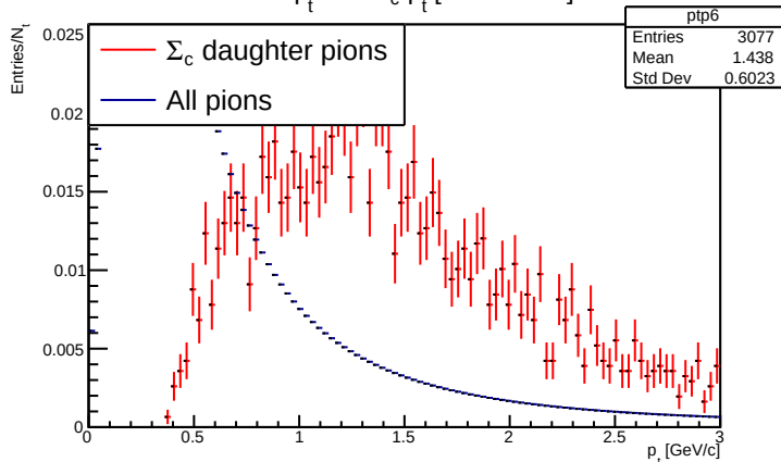
Pion p_t with \Sigma_c p_t [>12 GeV/c]
