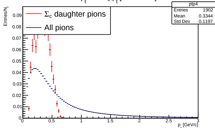
Pion p_t with \Sigma_c p_t [4-6 GeV/c]
