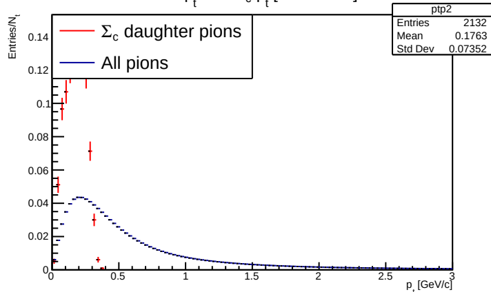
Pion p_t with \Sigma_c p_t [2-3 GeV/c]
