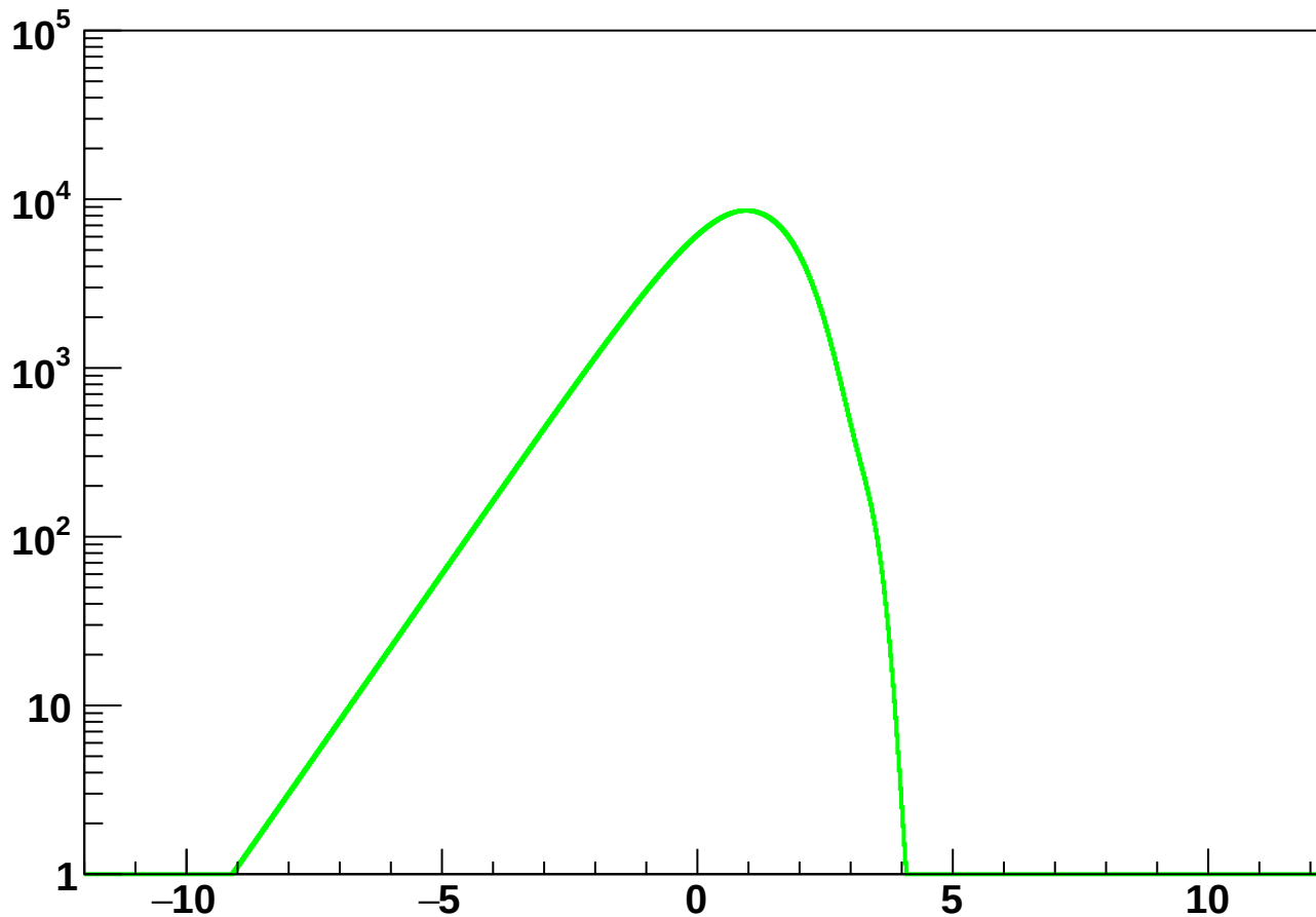
Signal \ln(\text{IP } \chi^2) PDF Projection
