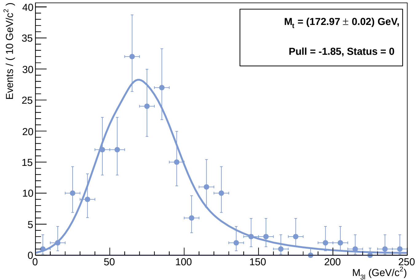
Mass of the combination of the reco J/\psi and the reco isolated lepton
