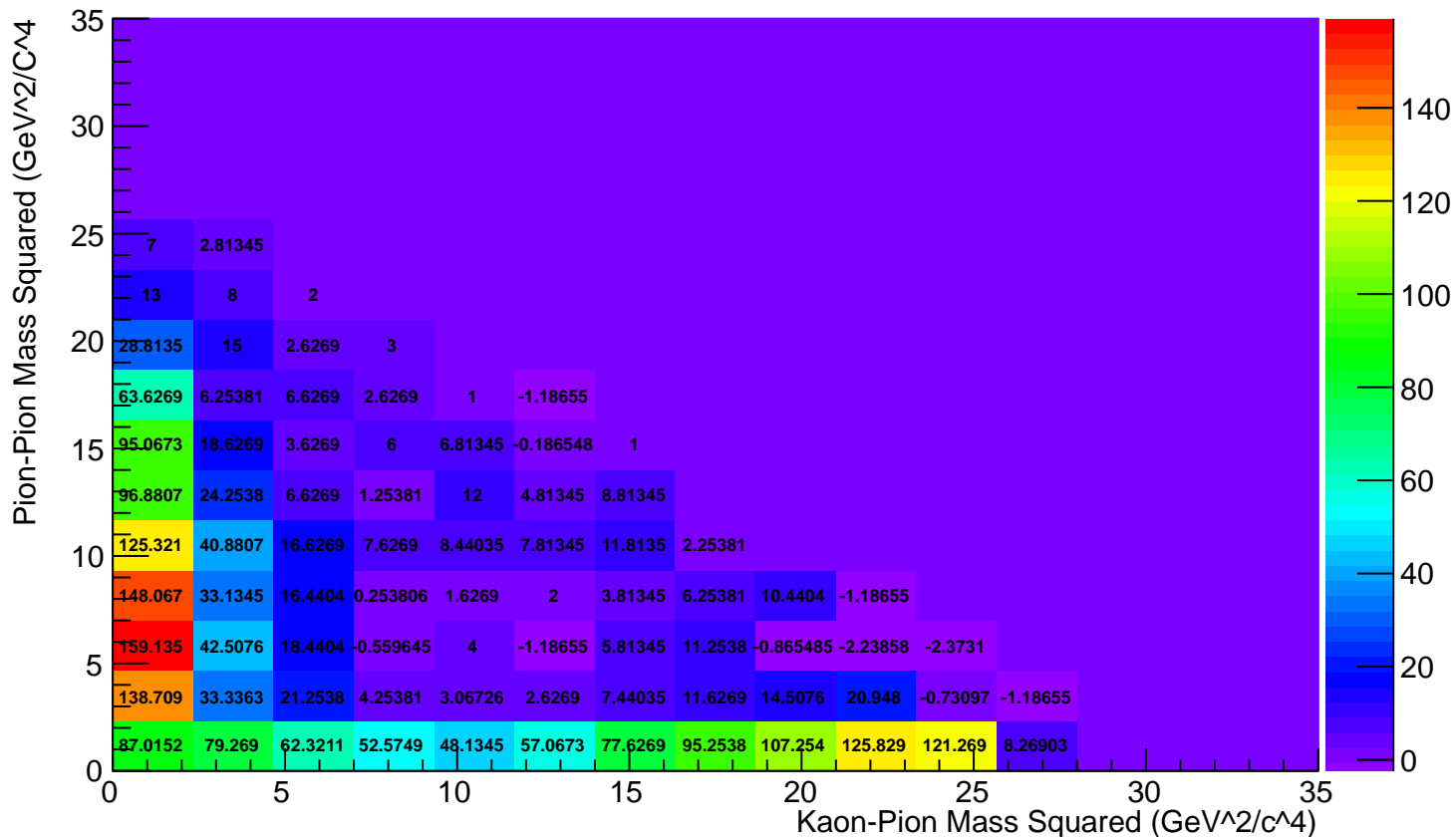
Dalitz Plot for negative signal data for both magnet orientations
