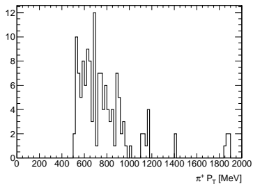
Figure: measured \pi^+ candidate p_T
