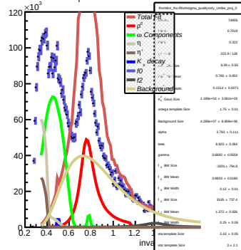
p T bin 0.6 - 1.0 GeV/c
