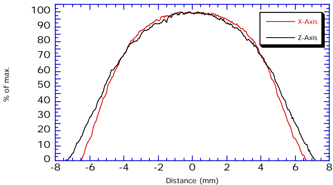
XZ Plane, 8mm Profiles
