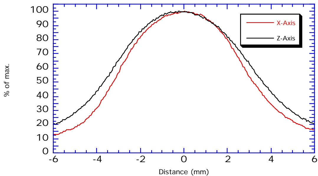
XZ Plane, 4mm Profiles
