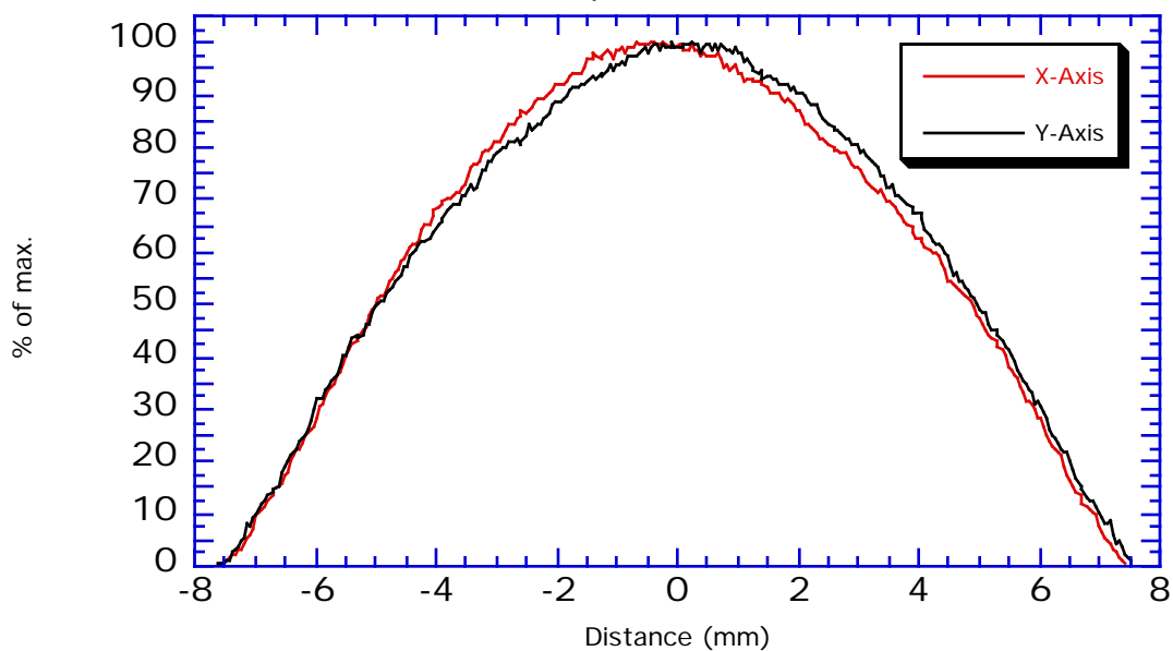
XY Plane, 8mm Profiles
